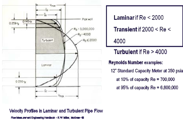
Figure 3 Flow profiles at various Reynolds numbers
