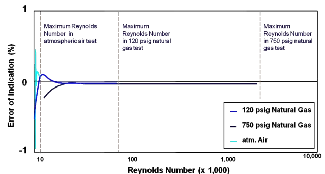
Figure 8 Turbine meter error vs Reynolds number
