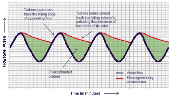
Figure 5 Intermittent flow response of turbine meter
