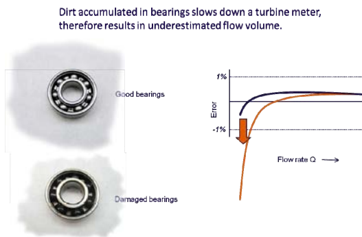
Figure 6 Impact of bearing damage on turbine meter
