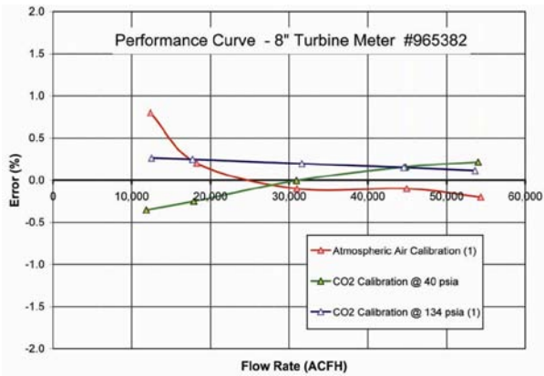
Figure 9 Line pressure effect on a turbine meter
