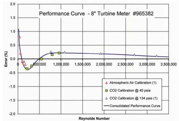
Figure 10 Calibration curve in Reynolds number
