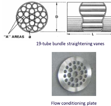
Figure 4 Tube bundle and flow conditioning plate
