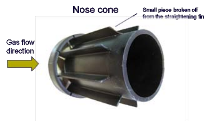
Figure 7 Laboratory tests showed that small damage on the nose cone resulted in a measurement error of nearly 2%
