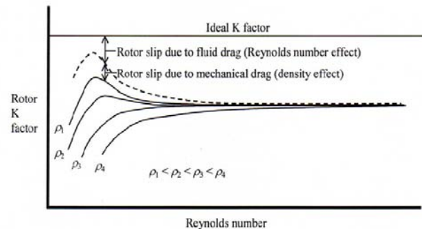
Figure 2 Effect of fluid and non-fluid retarding torques on gas turbine meter performance (Source: Sensus Metering Systems)
