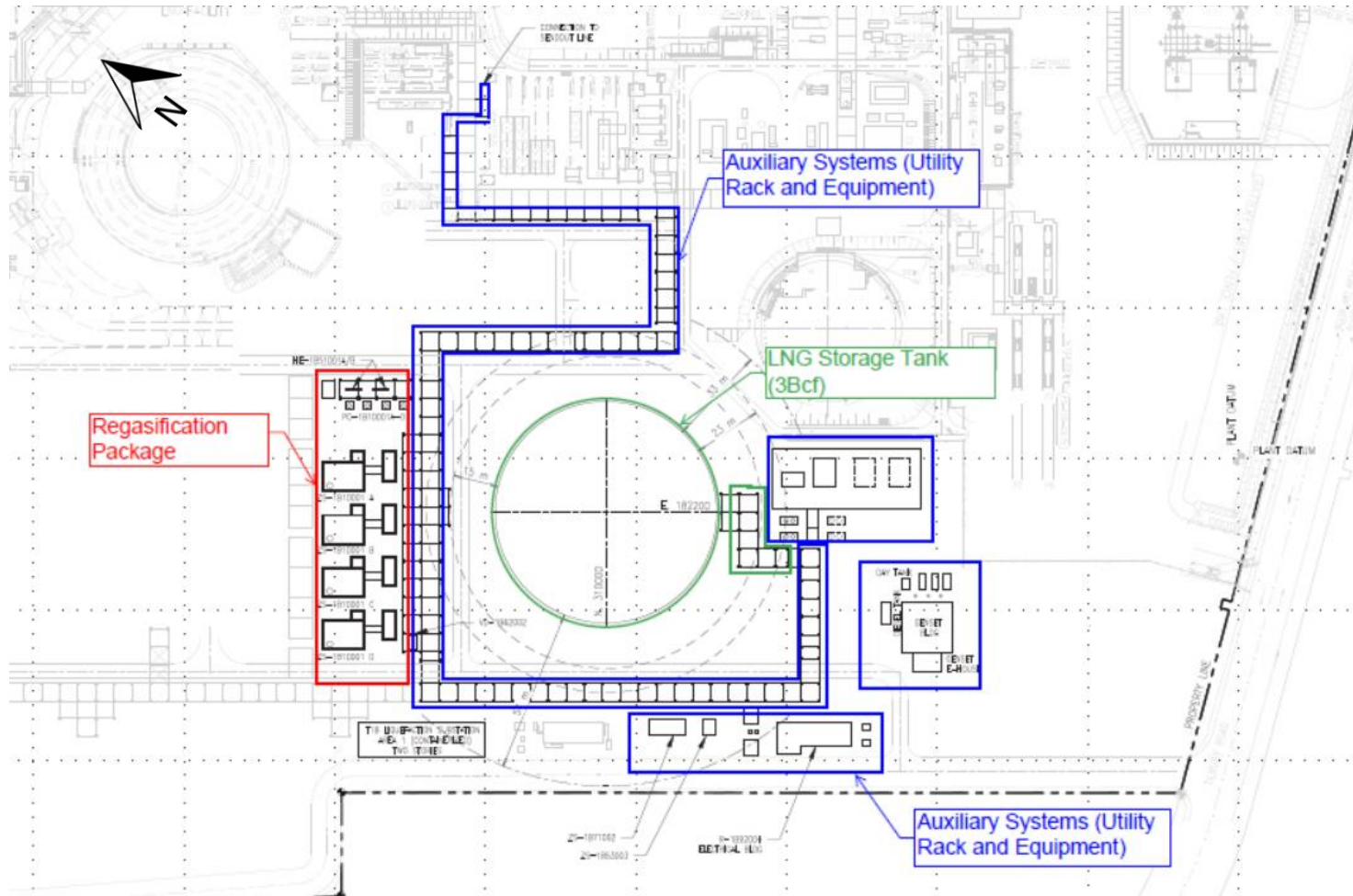
Figure 5-2: Proposed New Equipment Locations
